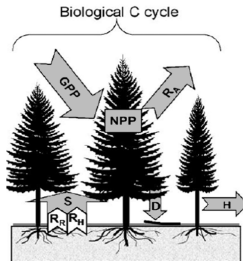
Figure 4.1 Diagram of the forest carbon cycle (Gower 2003).
