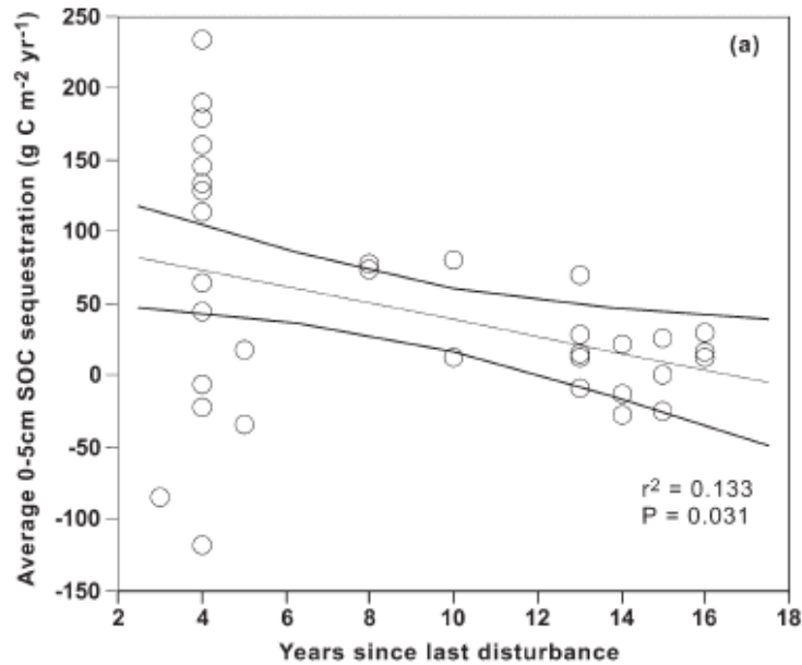
Figure 4.4 Changes in soil organic carbon (SOC) sequestration rate as a function of years since last disturbance. These prairies were planted on Alfisols and Mollisols. This graph shows the linear regression and the 95 percent confidence interval (modified from Kuckarik 2007).
