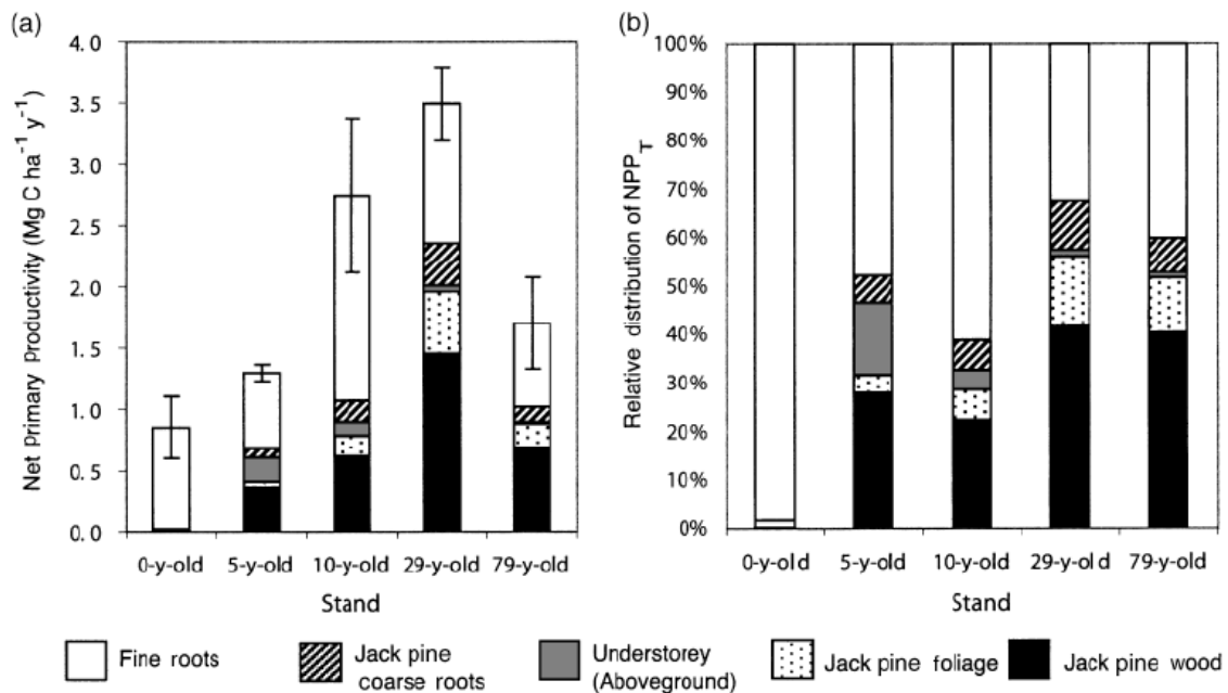
Figure 4.5 Allocation of carbon in (a) total NPP for stand and tissue type and (b) relative distribution of total NPP for tissue. These were from different aged jack pine stands in Saskatchewan, Canada (Howard, et al. 2004).
