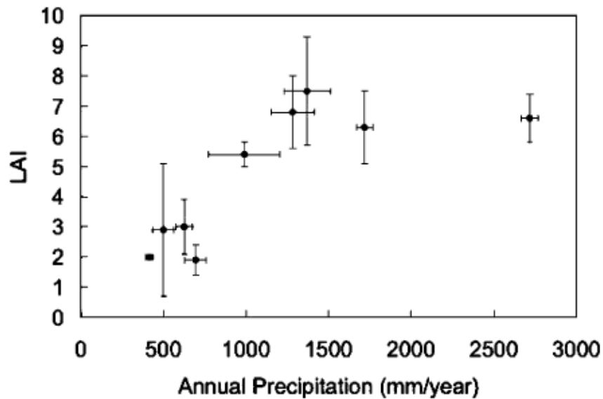
Figure 4.2 Relationship of average leaf area index (LAI) with annual precipitation (Gower 2003).
