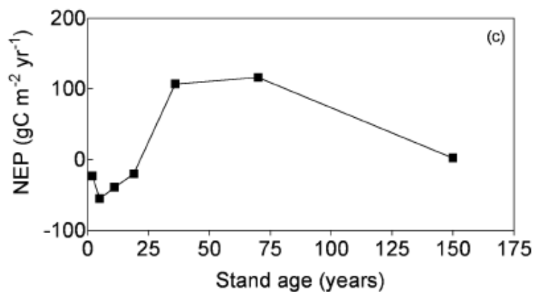
Figure 4.3 The net ecosystem production (NEP) for a well-drained boreal black spruce stand (modified from Gower 2003).
