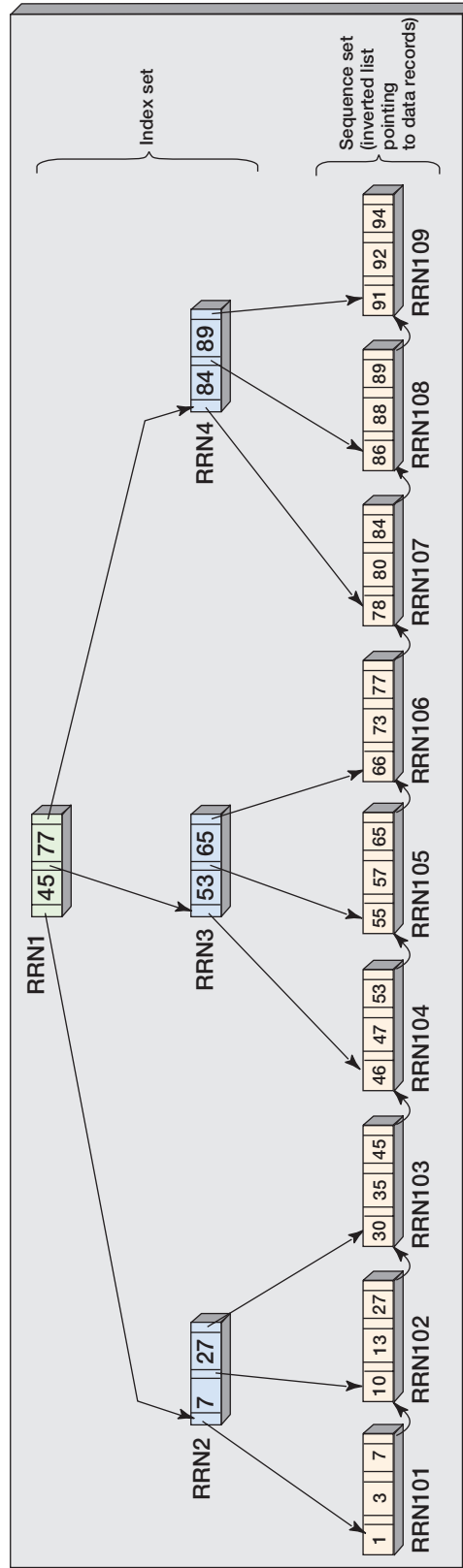
General Structure of a Simple B-Tree
