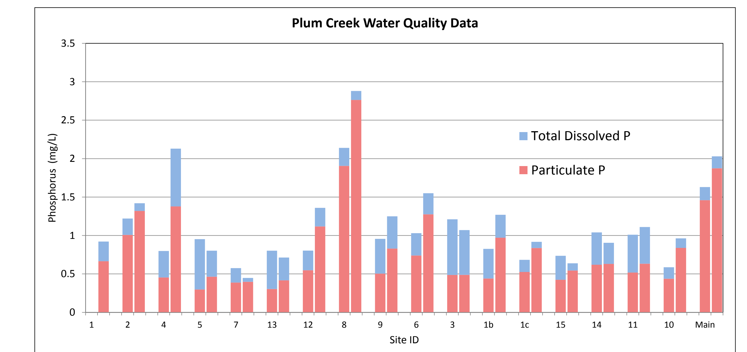
Figure 6. Phosphorus concentrations for 17 multi-field catchments and the main branch of Plum Creek from April 16 and April 26, 2011 events. There is a range of P concentration in runoff among sites. The differences appear to be related to STP, cover and slope. More data is needed to explore these relationships (Figure 7).
