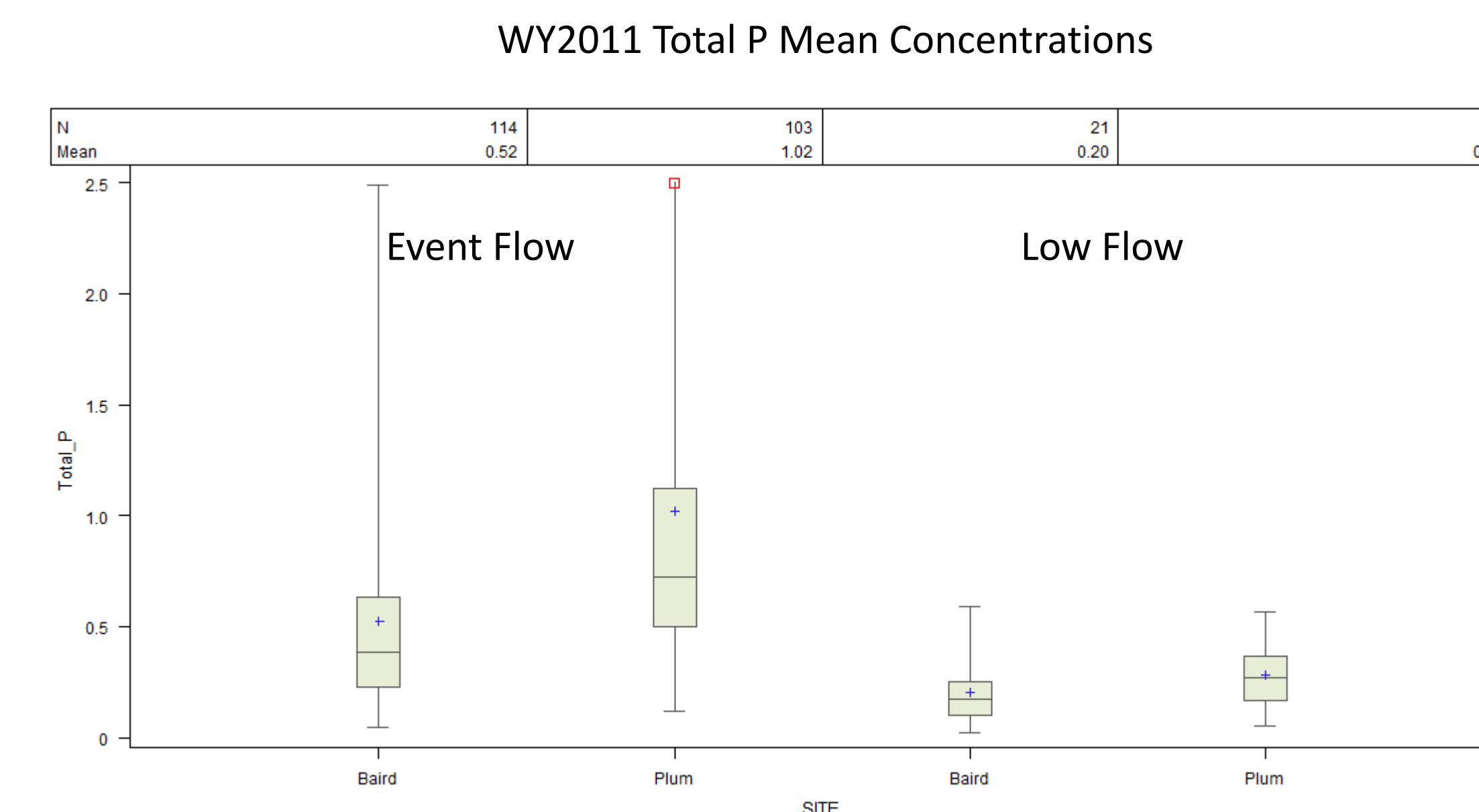
Figure 3. WY2011 Event and low flow TP concentrations (mg/L) for Baird and Plum Creeks. Box plot show range, interquartile range, mean (+) and median (—) concentrations. Higher P loss in Plum likely a result of agricultural intensity (Figure 1). Event flow TP mean concentrations for Plum Creek were significantly greater than Baird Creek ( p \leq 0.05 ). All mean and median concentrations are well above target of 0.075 mg/L TP.
