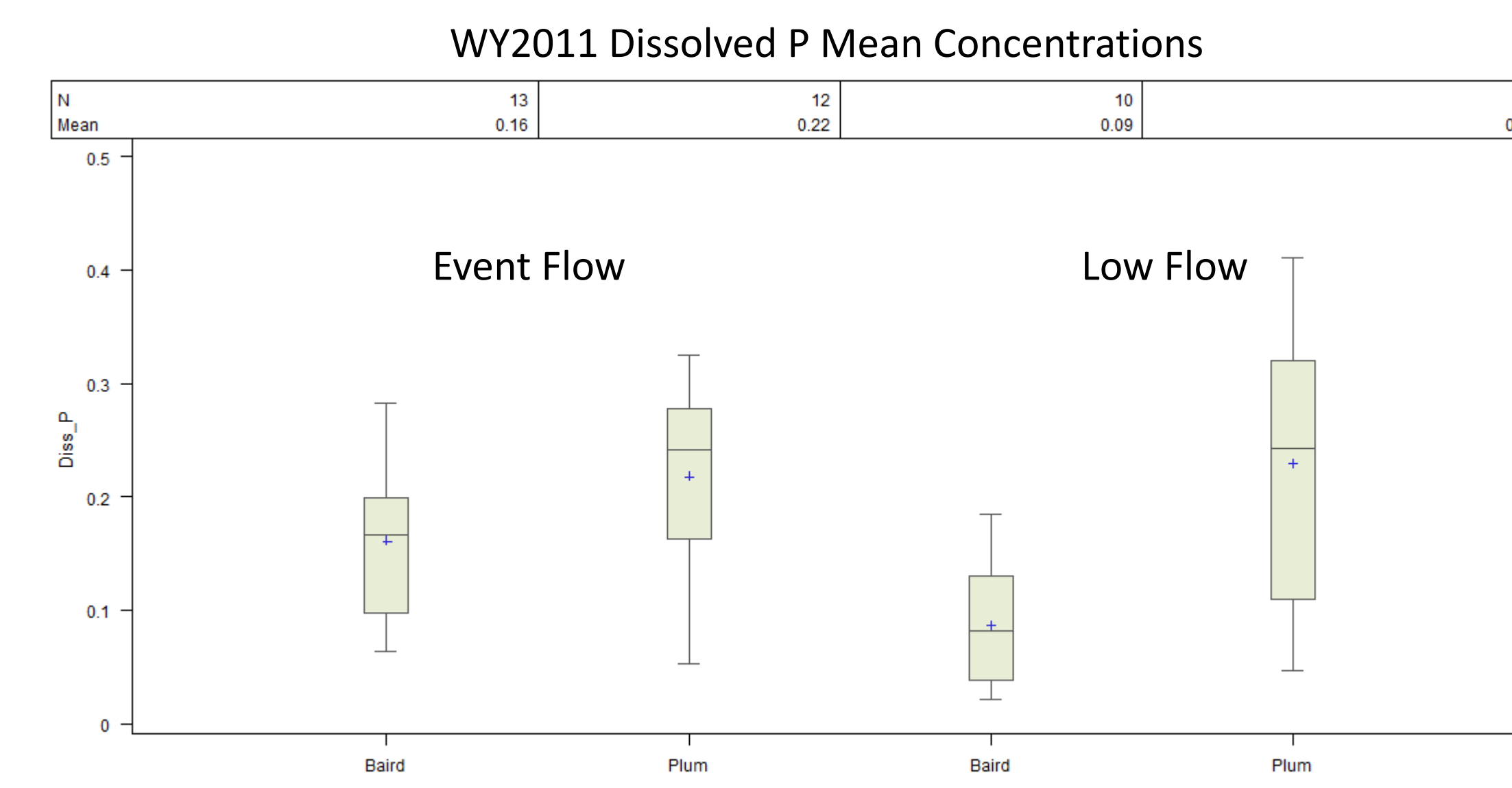
Figure 4. WY2011 Event and low flow DP concentrations (mg/L) for Baird and Plum Creeks. Box plot show range, interquartile range, mean (+) and median (—) concentrations. Higher P loss in Plum likely a result of agricultural intensity (Figure 1). Low flow DP mean concentrations for Plum Creek were significantly greater than Baird Creek ( p \leq 0.05 ).
