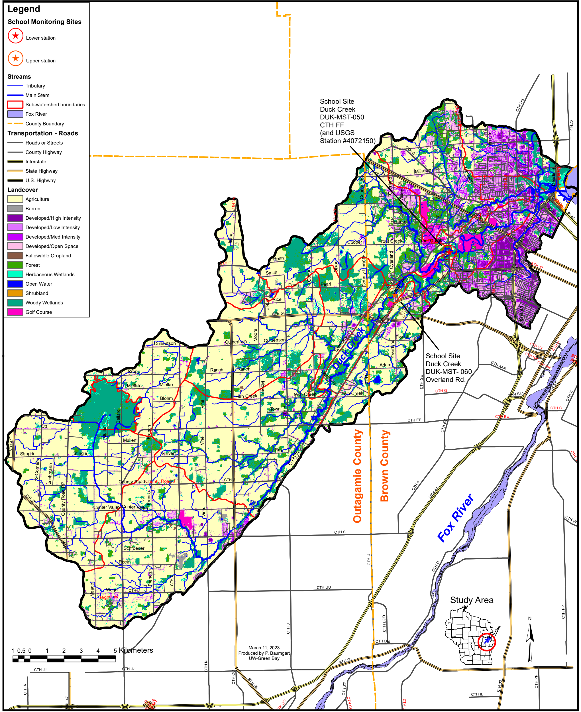
Land cover and landuse in the 392 sq. km Duck Creek watershed. Image based on USDA National Agricultural Statistics Service 2022 Cropland Data Layer, published crop-specific data layer [Online].
