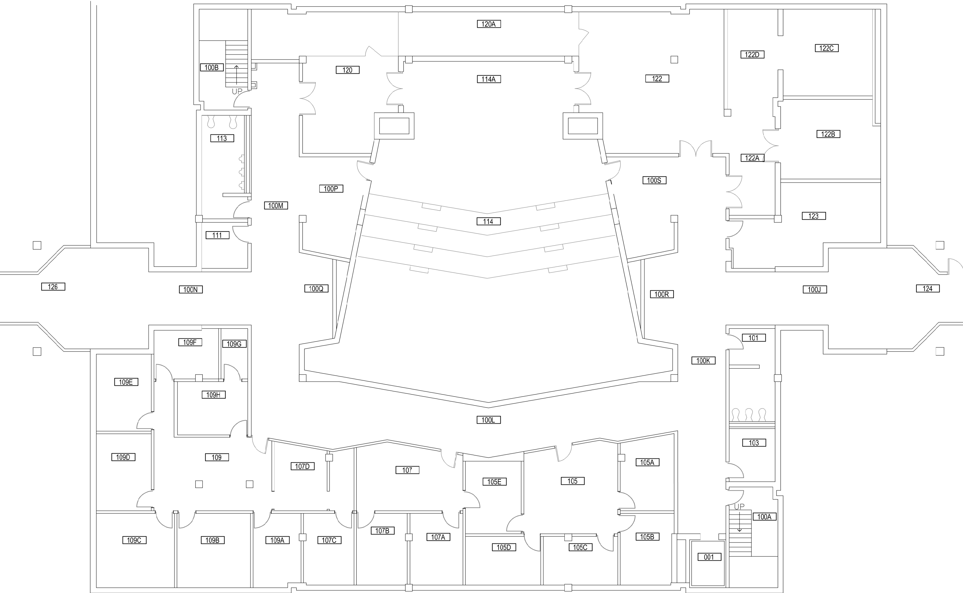
Environmental Science Building - 1st Floor
